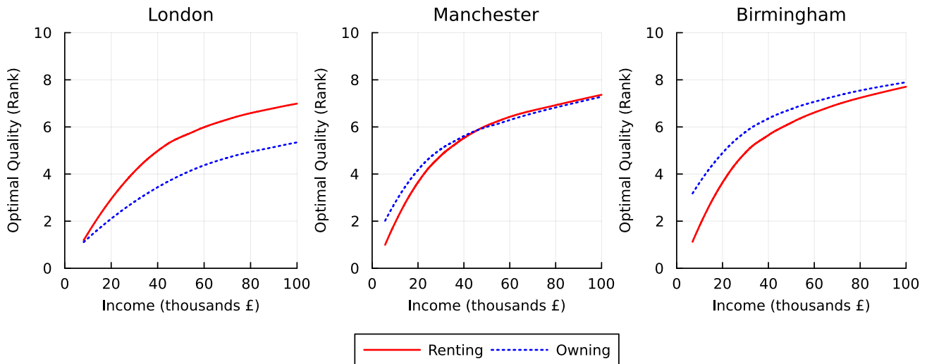
Figure A14: Average Unconstrained Optimal Quality by Tenure and Income
